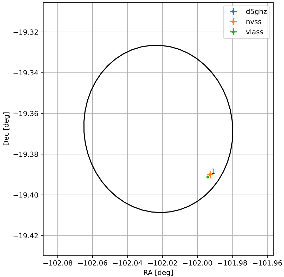
4FGL J1711.9-1922
