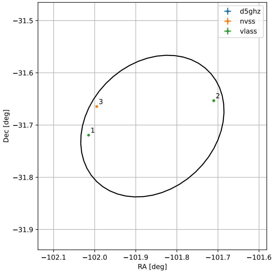
4FGL J1712.5-3142
