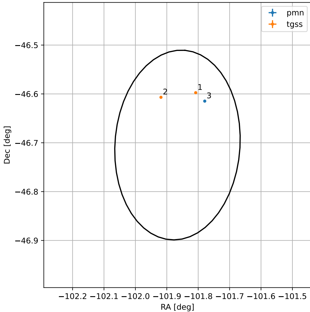
4FGL J1712.5-4642
