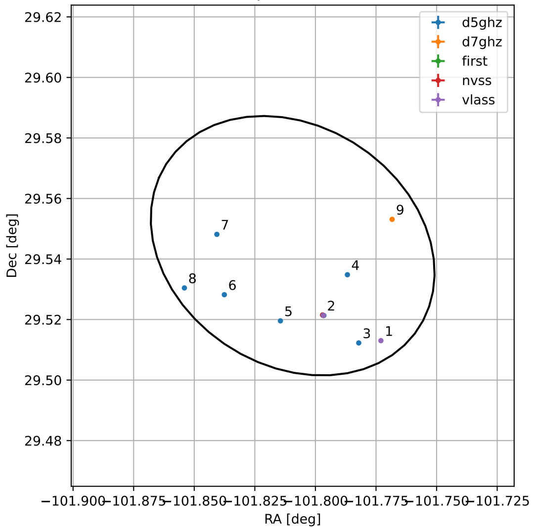
4FGL J1712.7+2932
