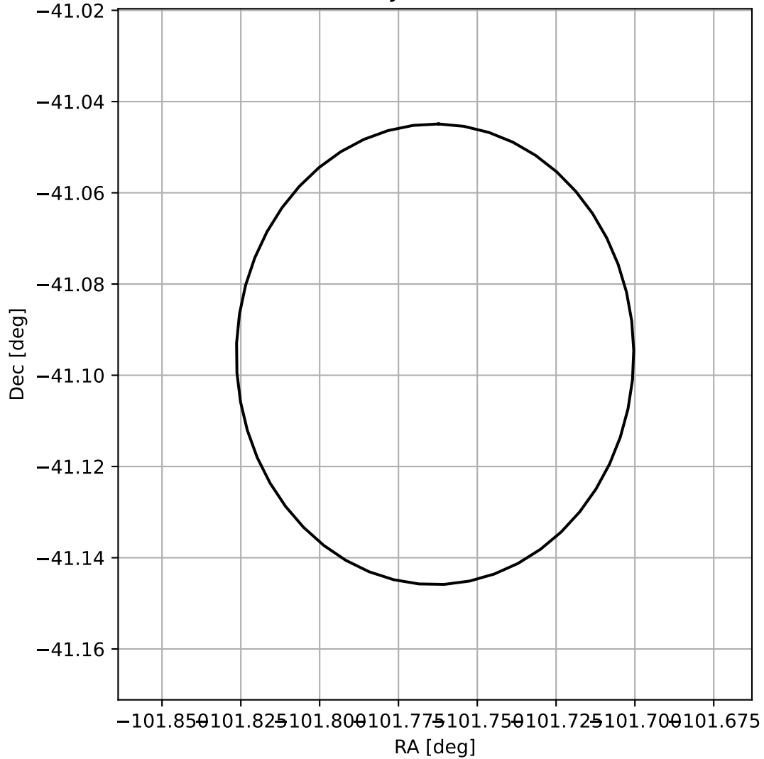
4FGL J1712.9-4105
