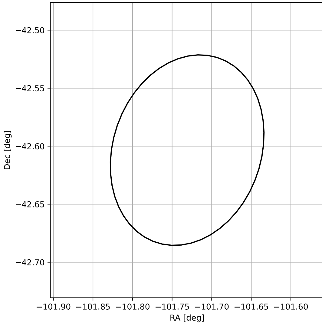
4FGL J1713.0-4236
