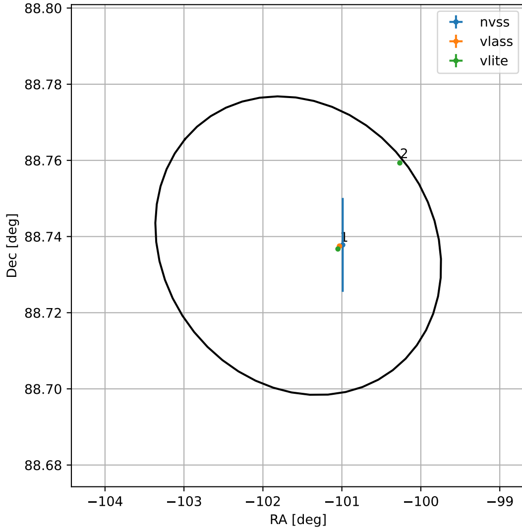
4FGL J1713.7+8844
