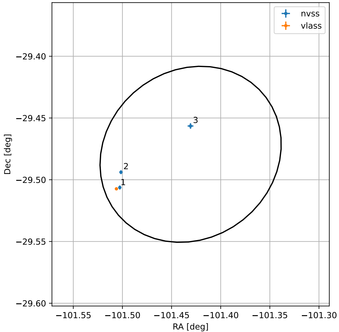
4FGL J1714.2-2928
