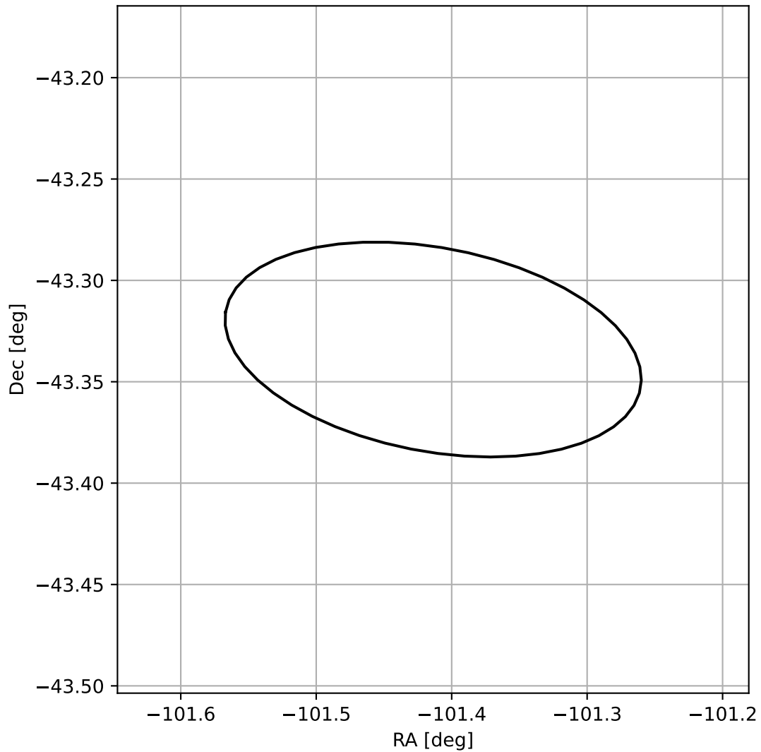
4FGL J1714.3-4320
