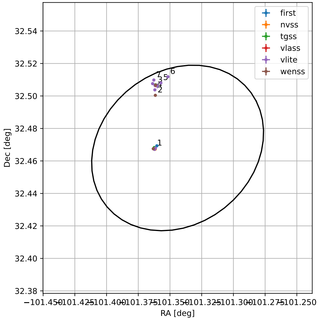
4FGL J1714.6+3228
