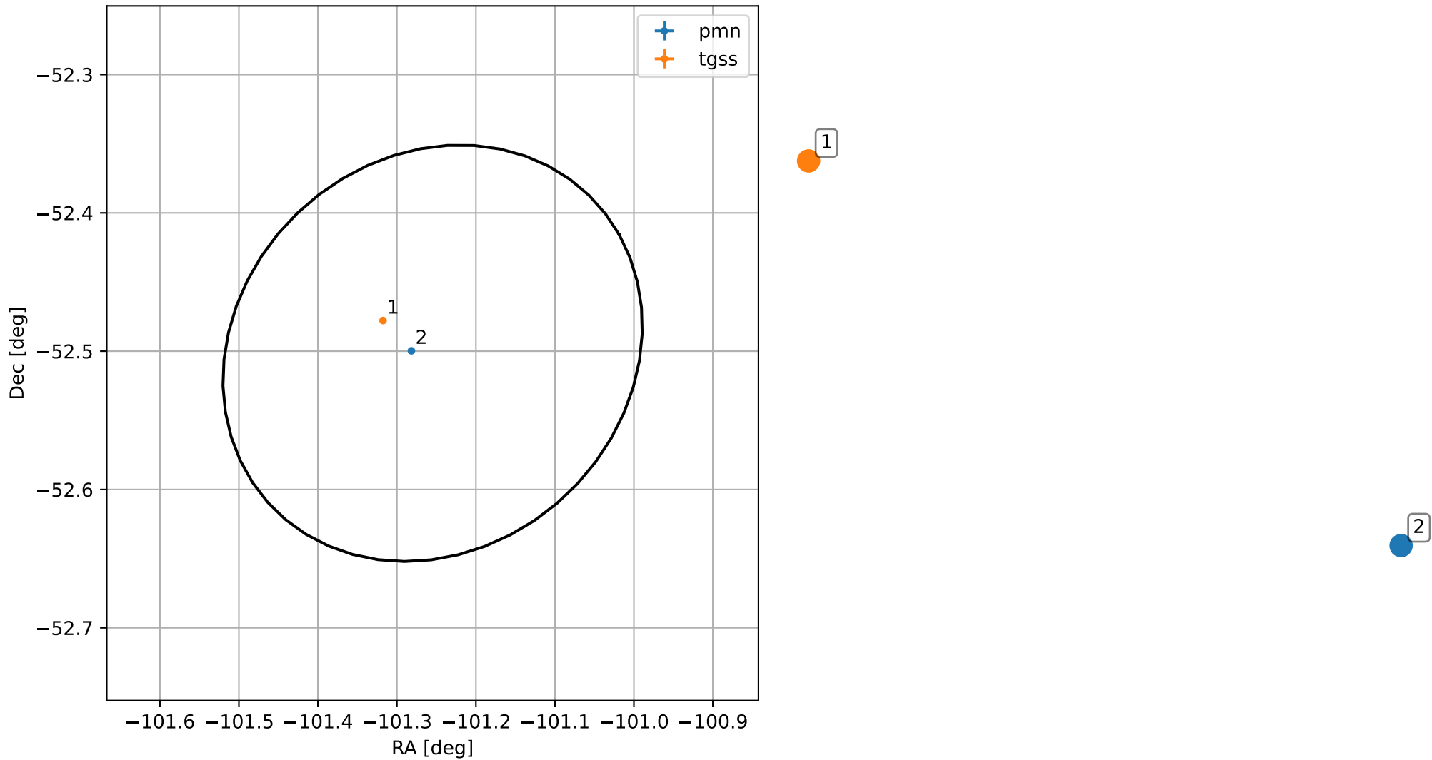
4FGL J1714.9-5230
