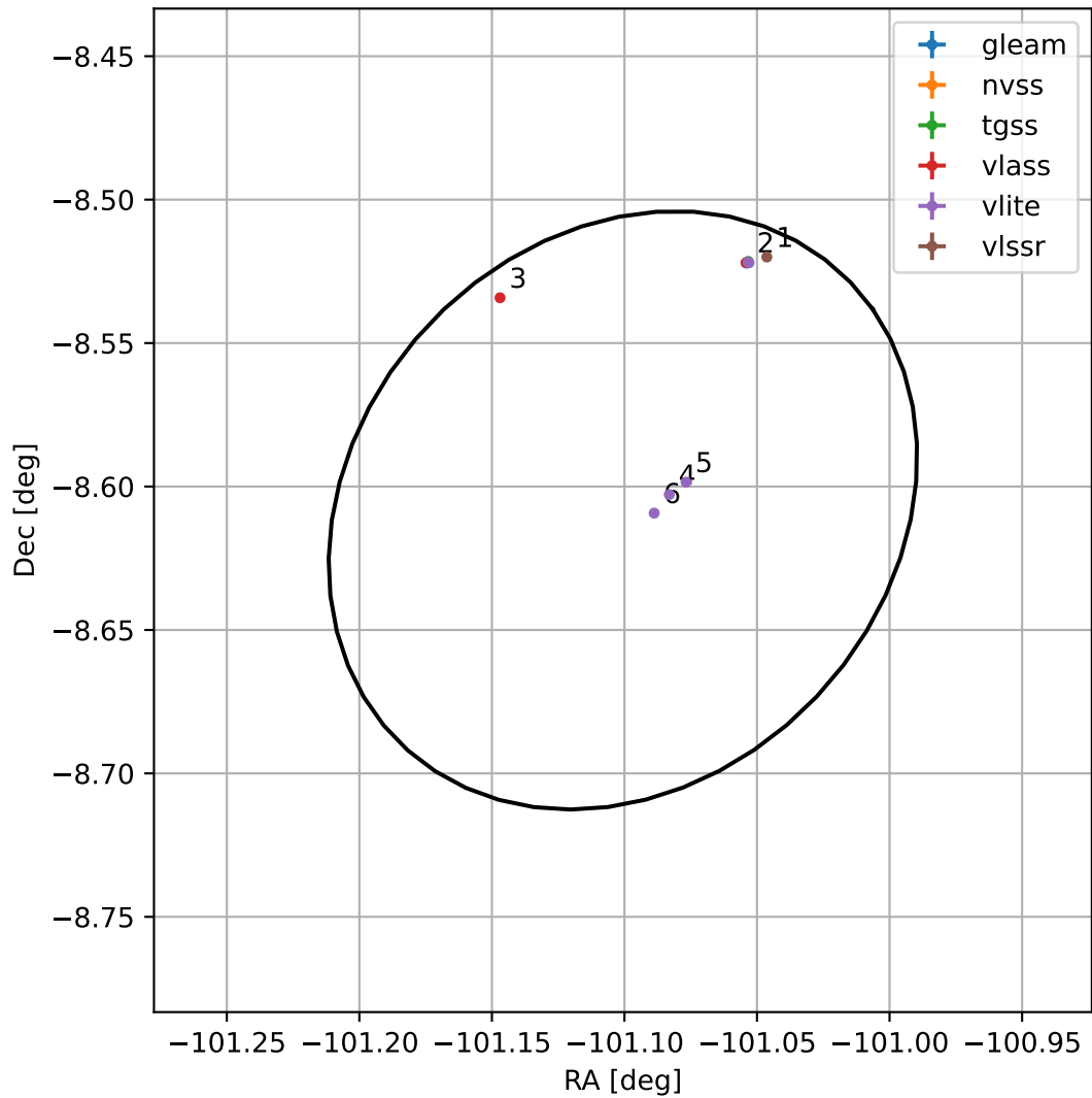
4FGL J1715.5-0836
