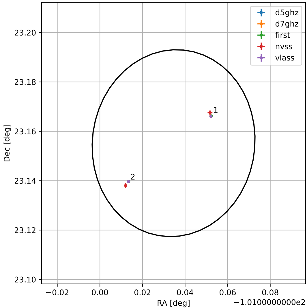
4FGL J1716.1+2309
