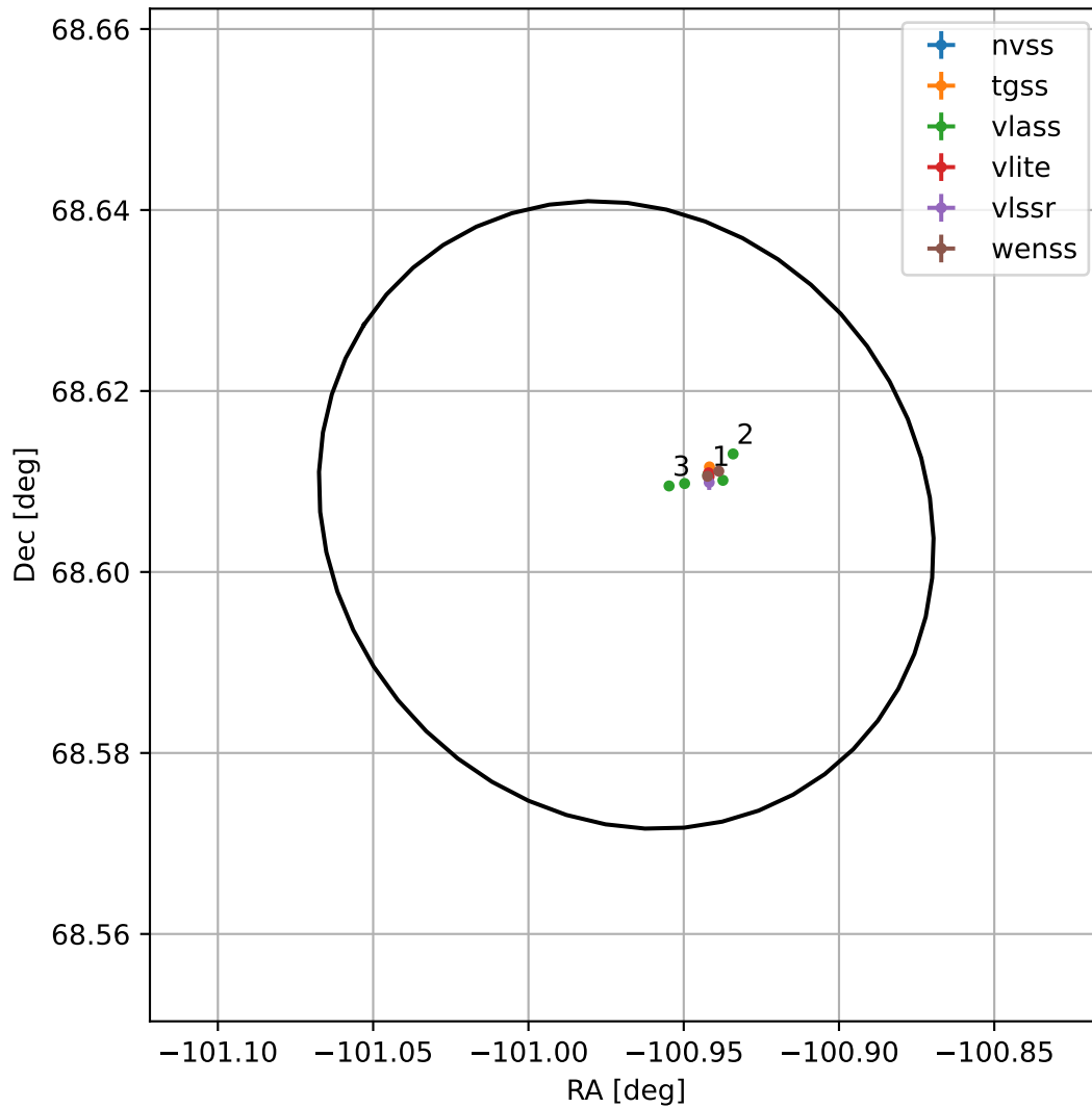
4FGL J1716.1+6836
