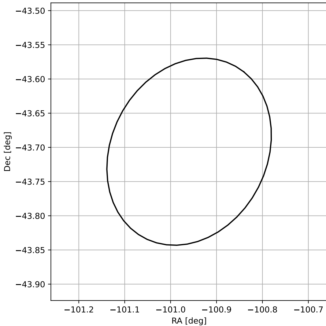
4FGL J1716.1-4342
