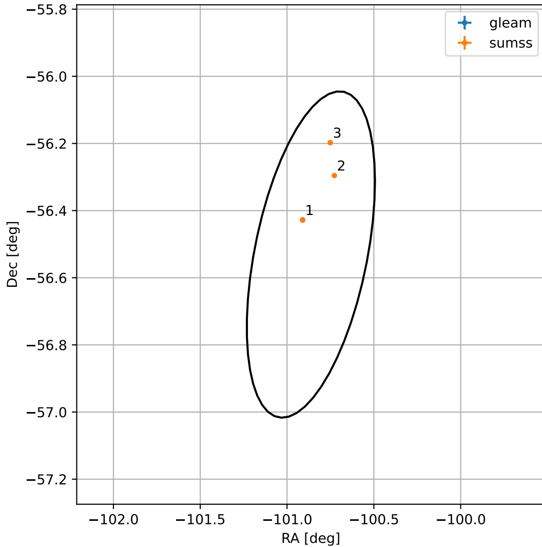
4FGL J1716.5-5631
