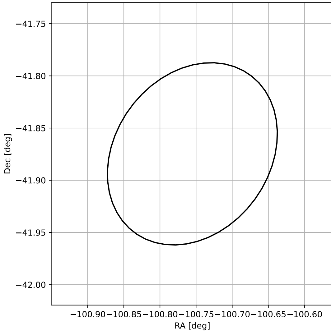
4FGL J1716.9-4152
