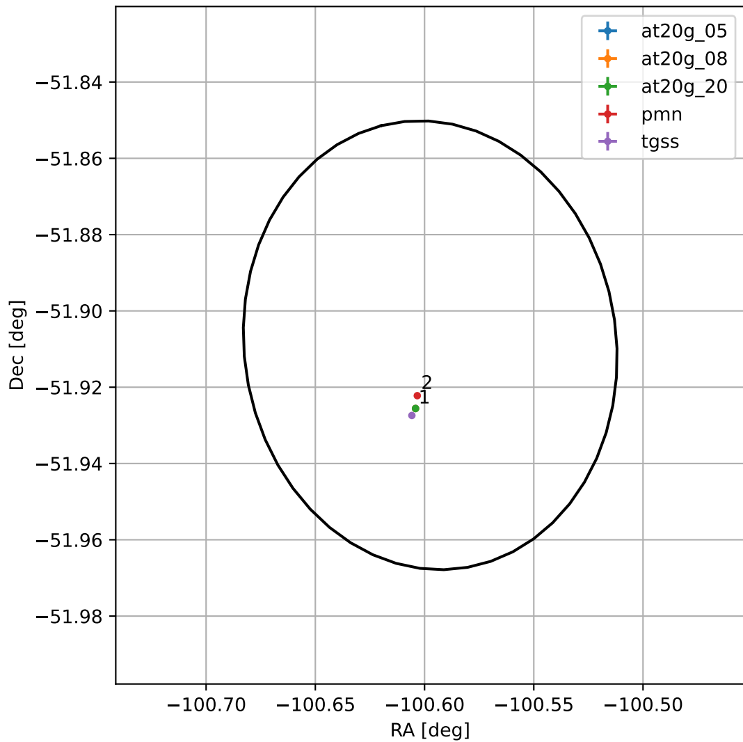
4FGL J1717.6-5154
