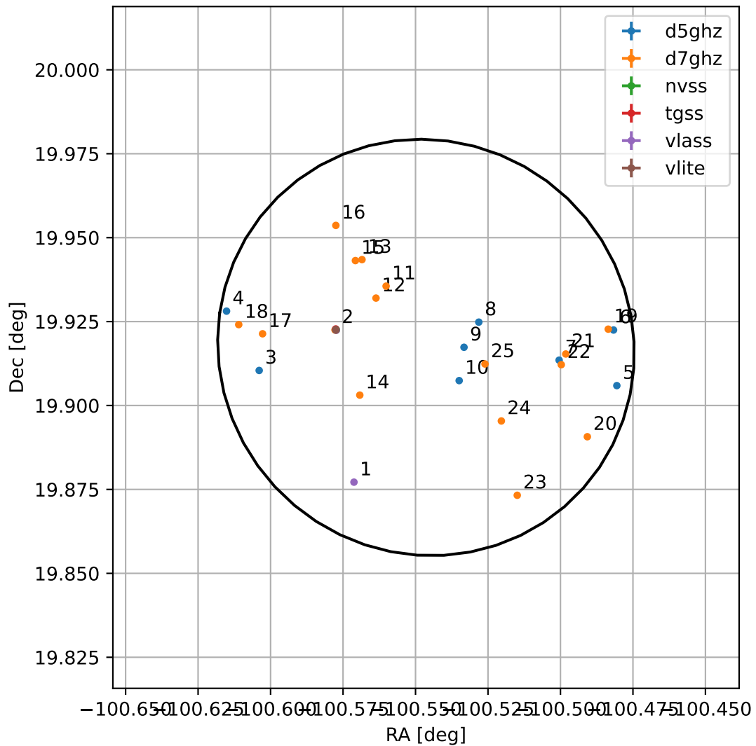
4FGL J1717.8+1955
