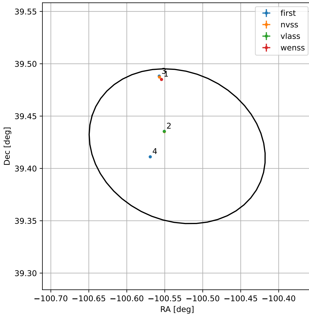
4FGL J1717.8+3925
