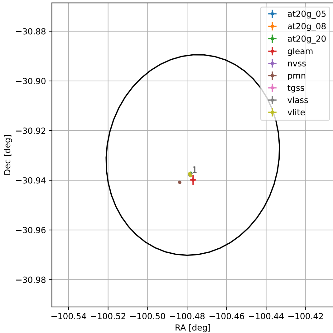
4FGL J1718.0-3055
