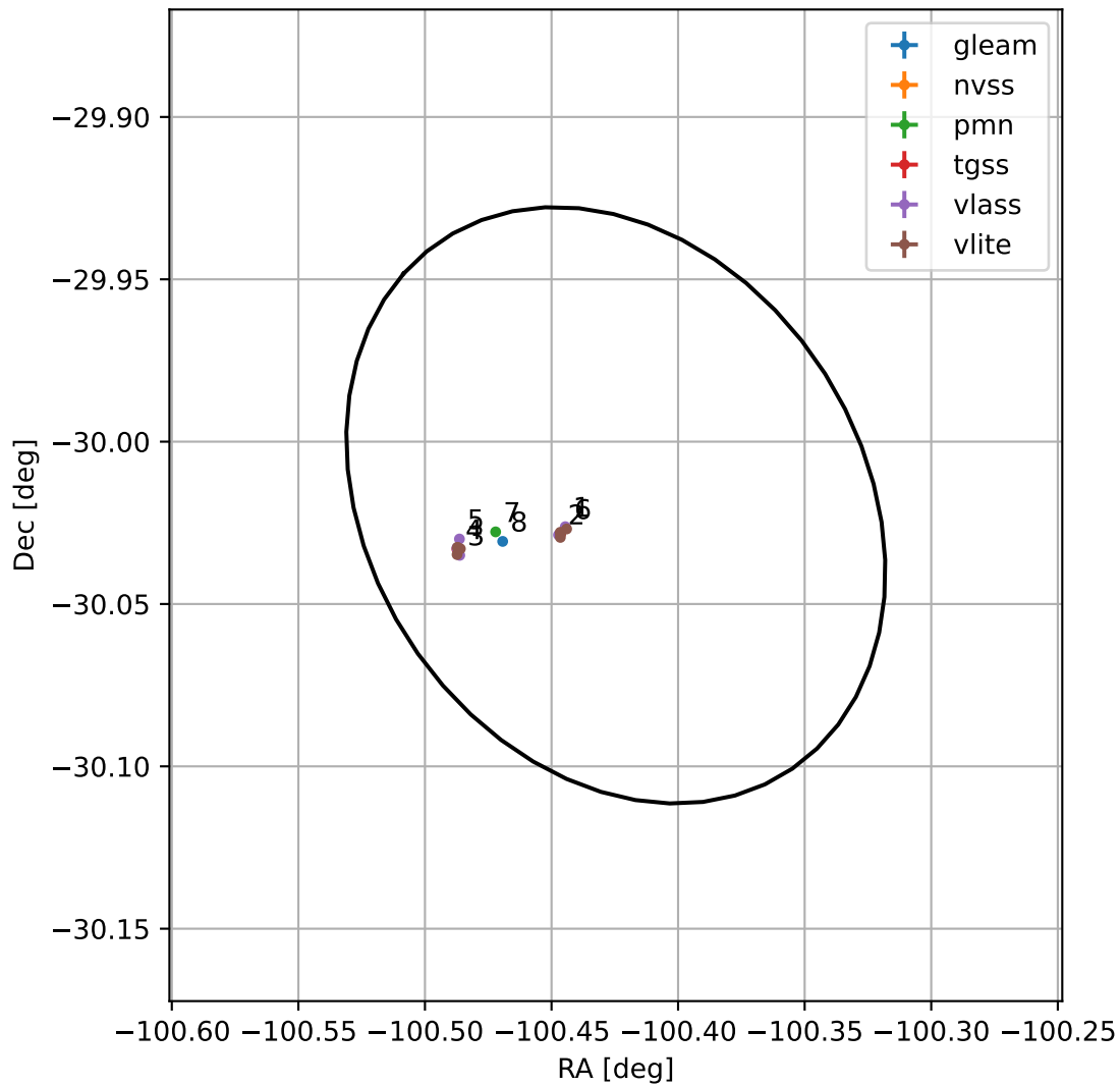
4FGL J1718.3-3001
