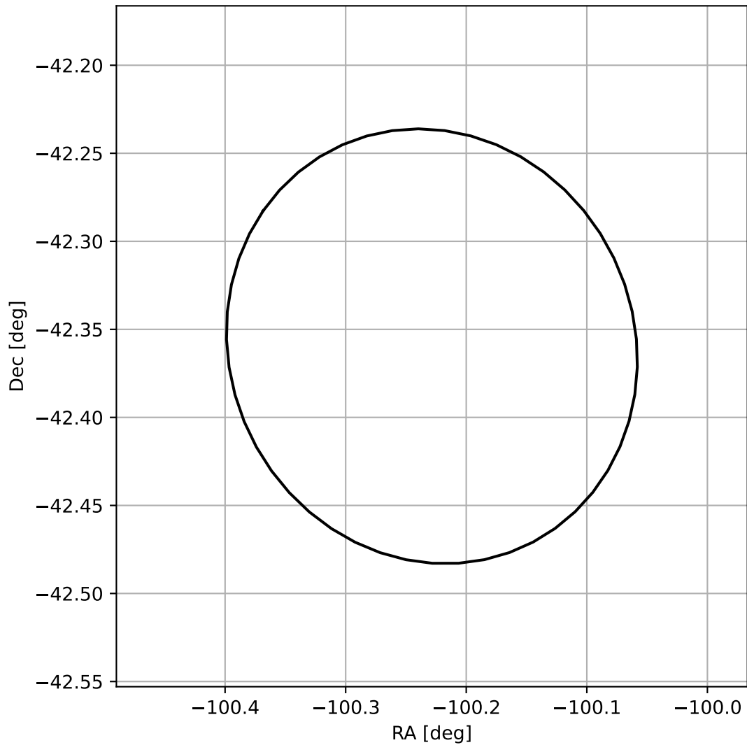
4FGL J1719.0-4221
