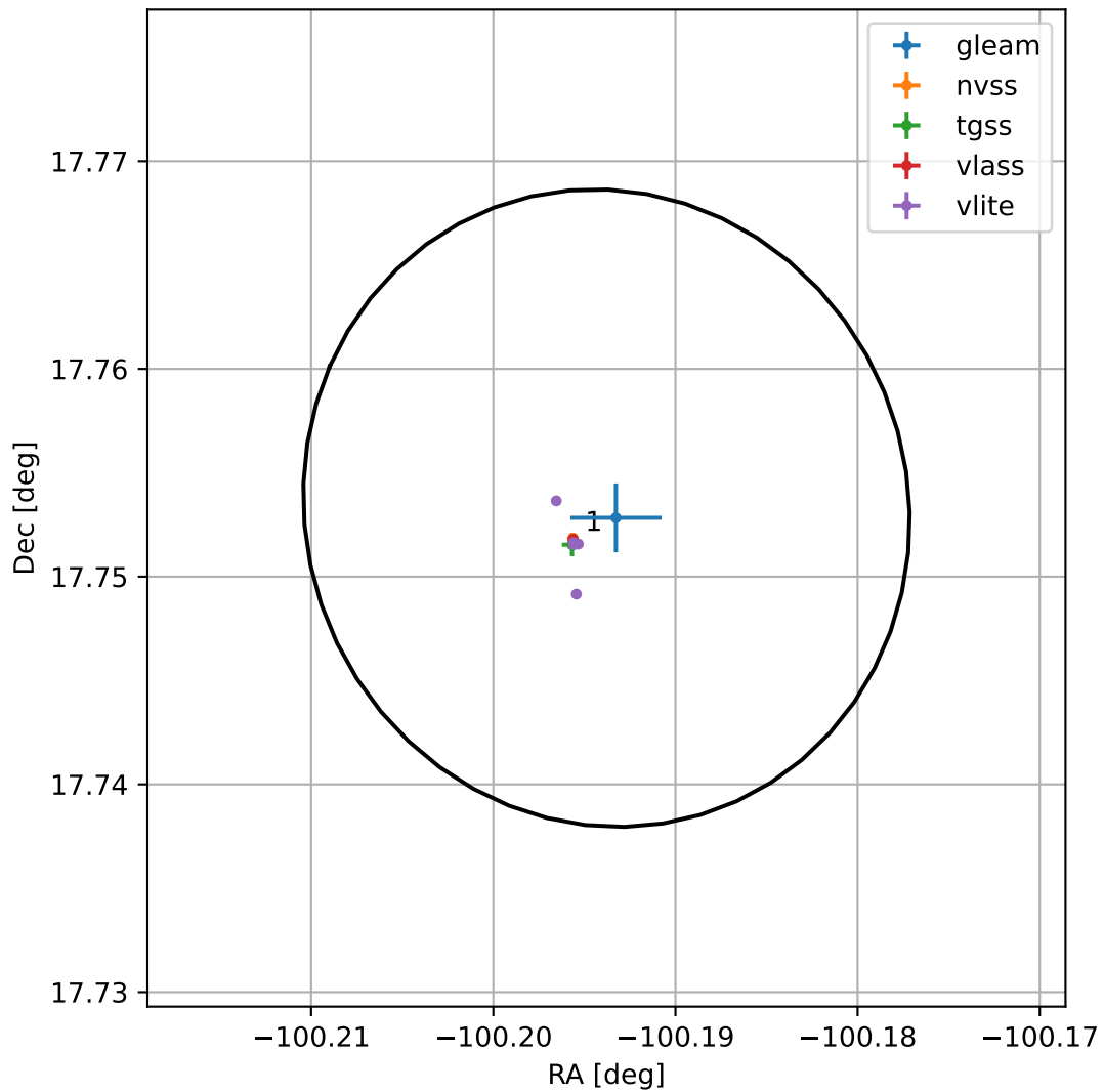
4FGL J1719.2+1745
