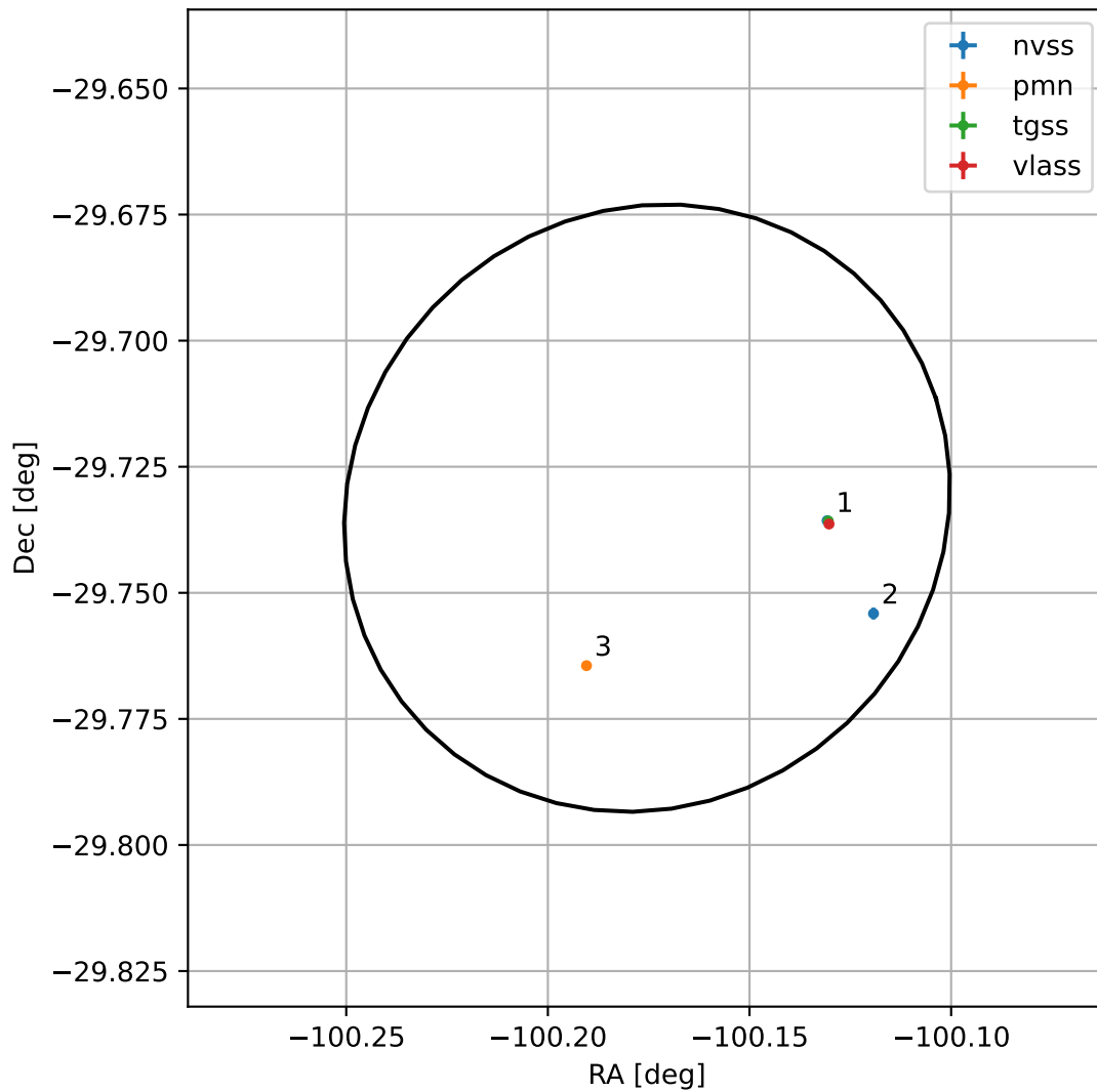
4FGL J1719.2-2943
