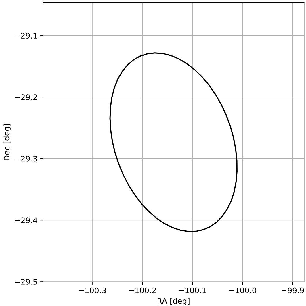
4FGL J1719.4-2916
