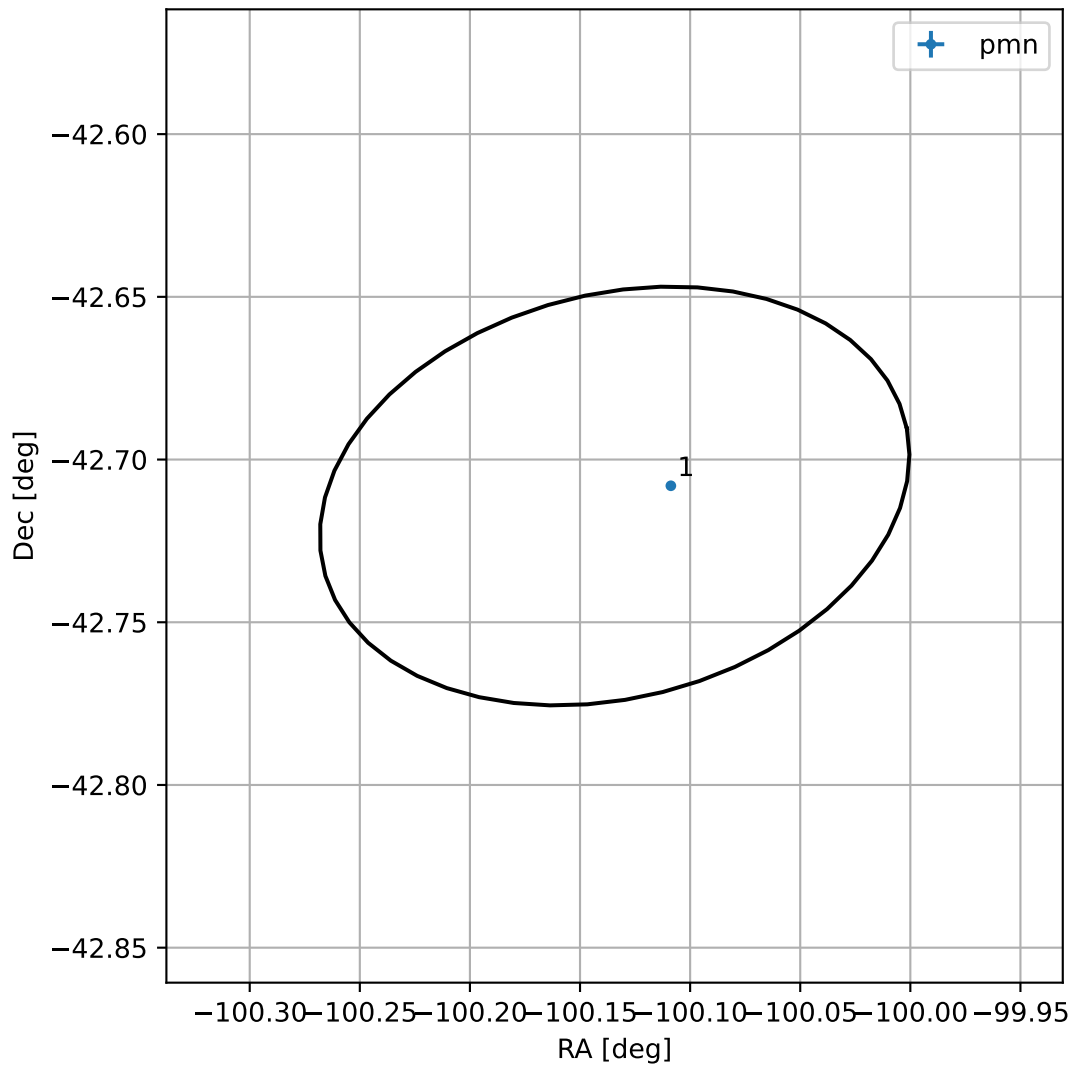
4FGL J1719.4-4242
