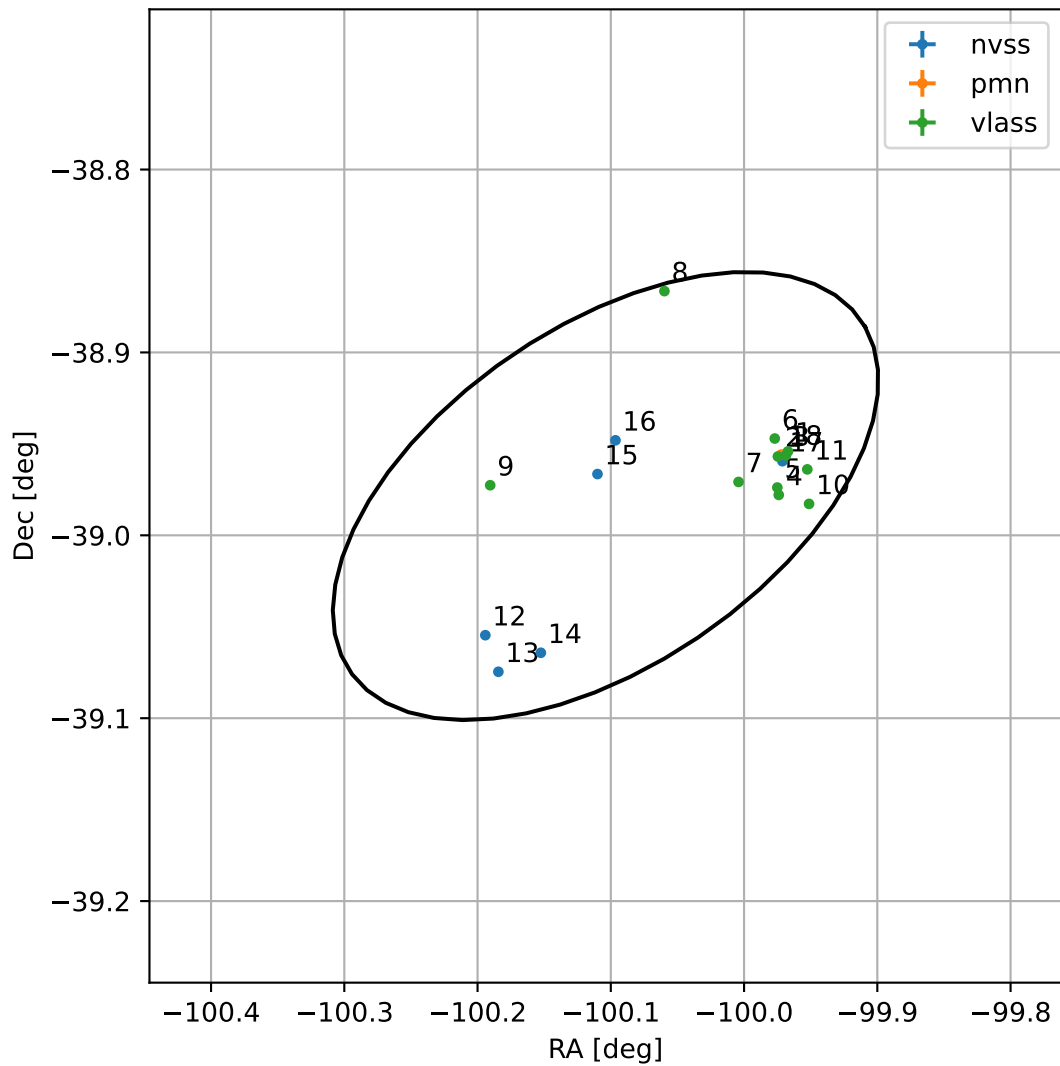
4FGL J1719.5-3858
