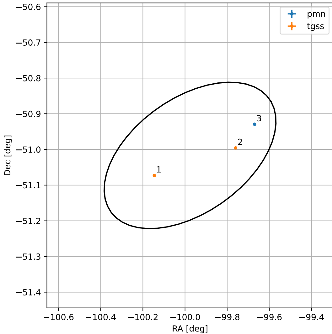
4FGL J1720.0-5101
