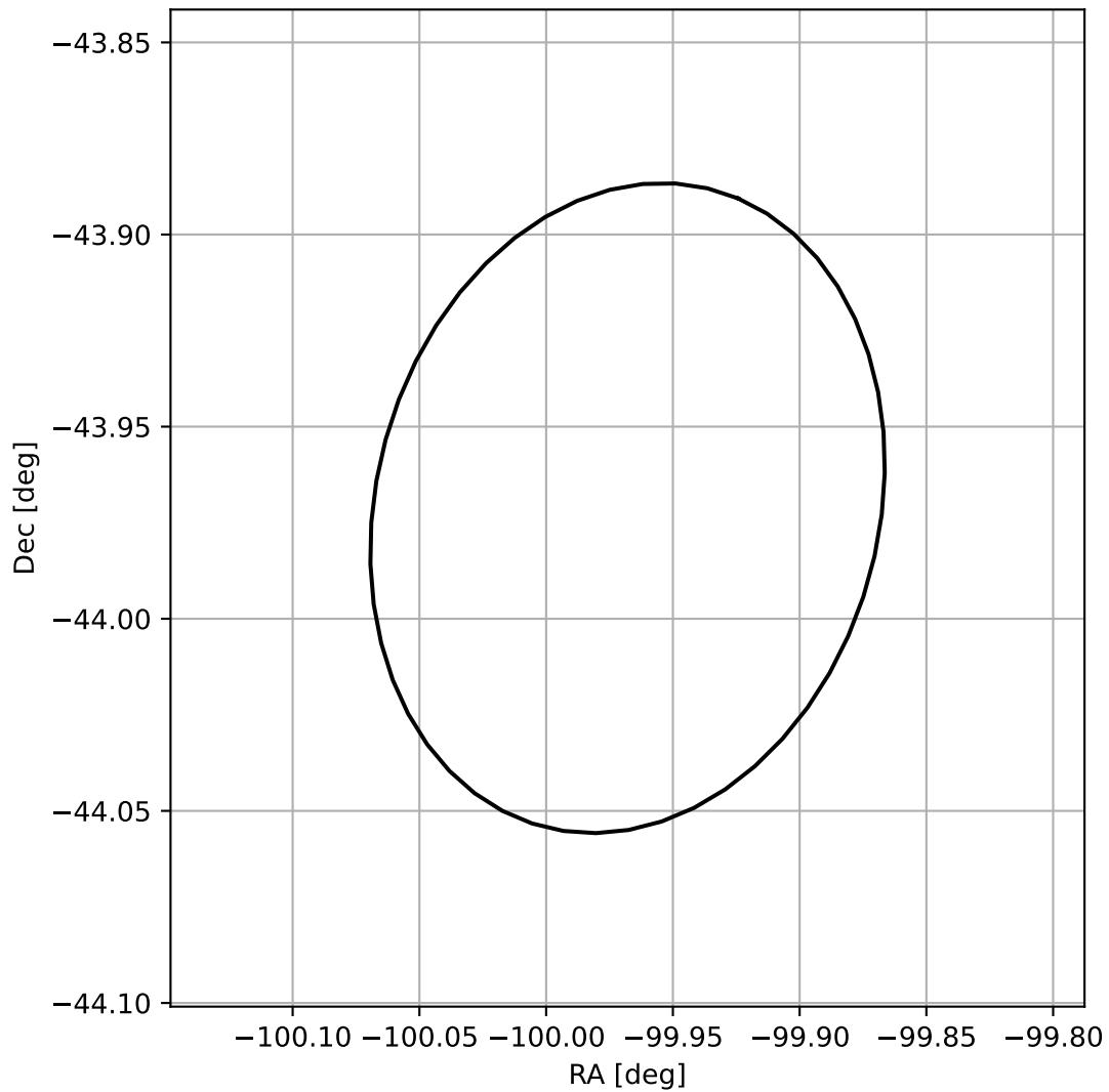
4FGL J1720.1-4358
