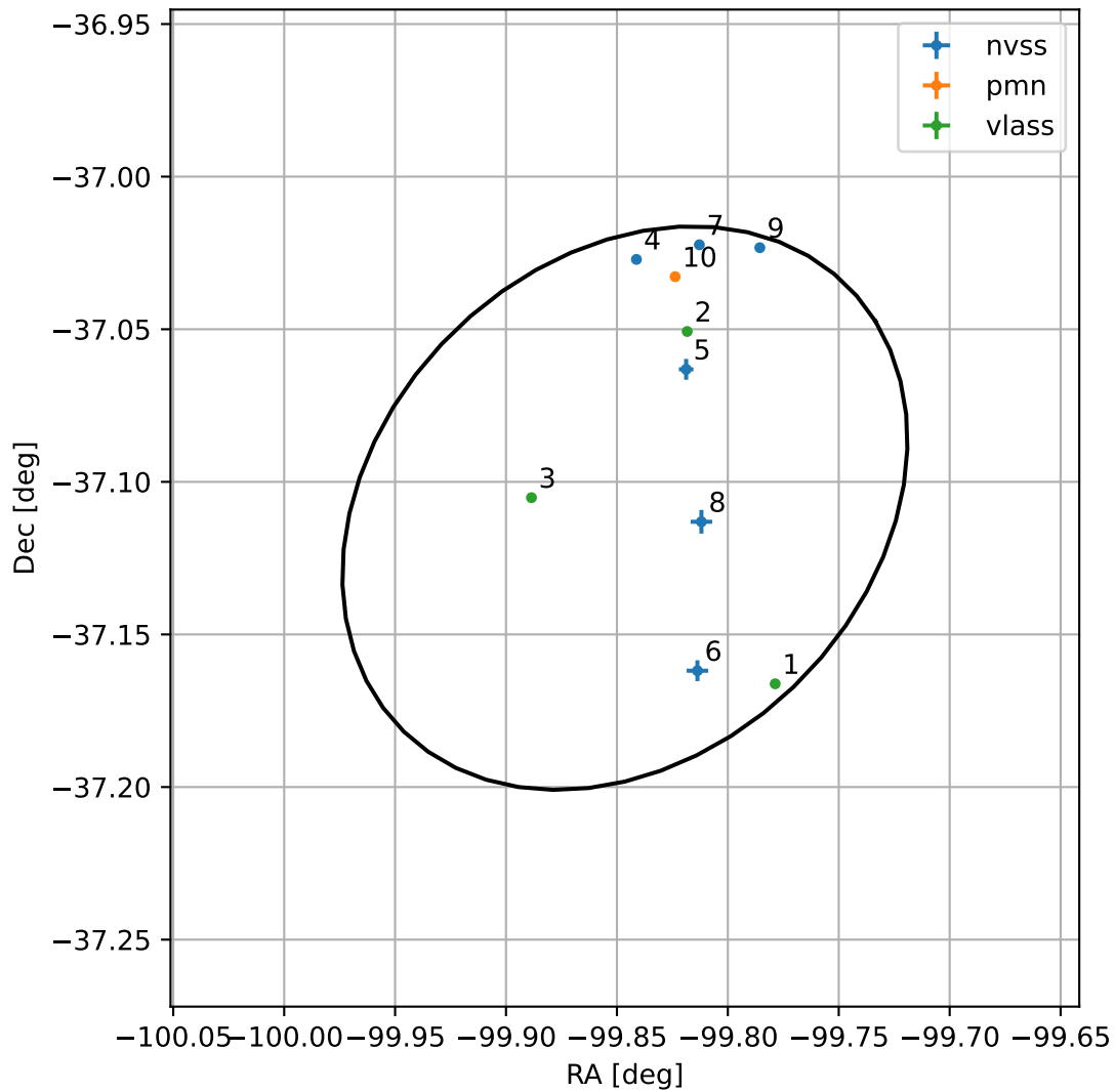
4FGL J1720.6-3706
