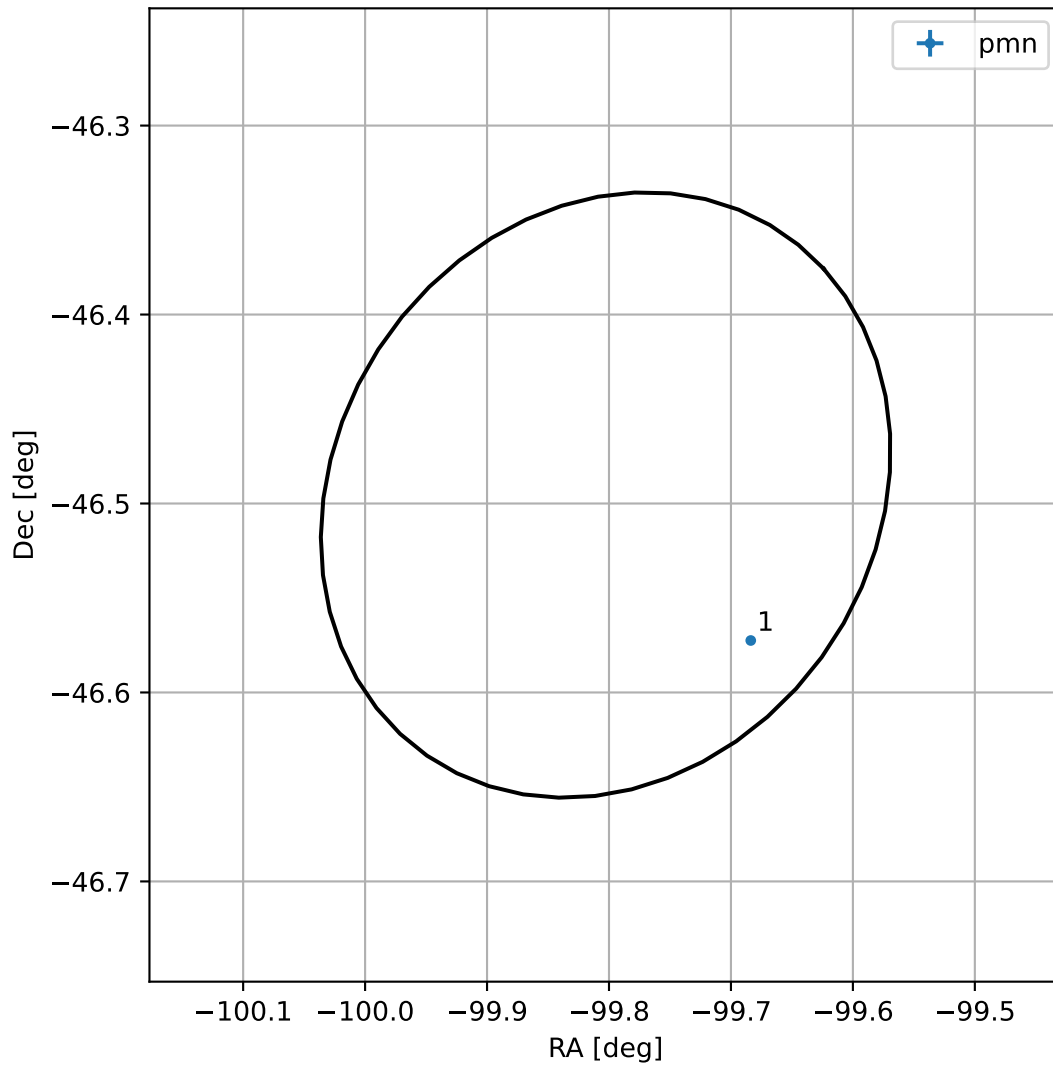
4FGL J1720.7-4629
