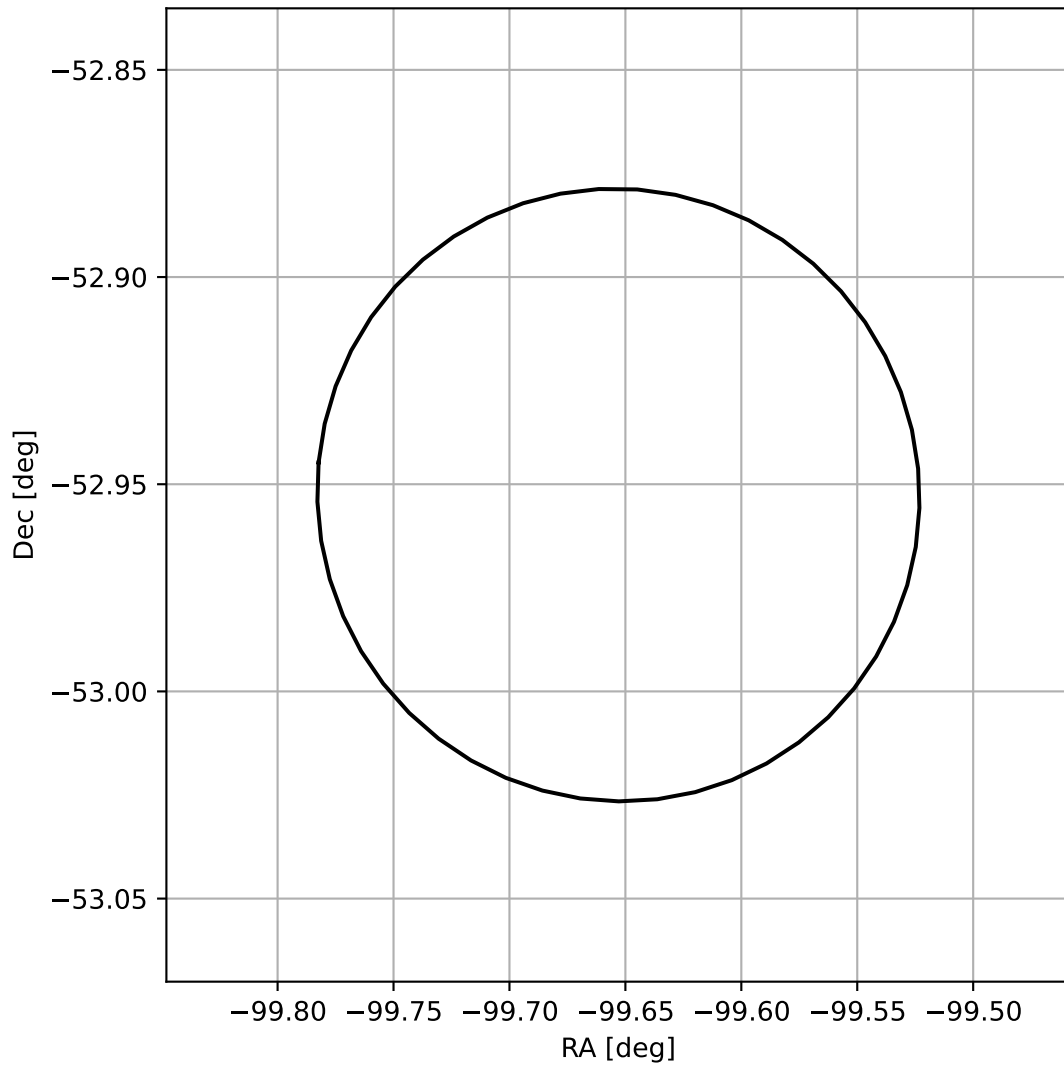
4FGL J1721.3-5257
