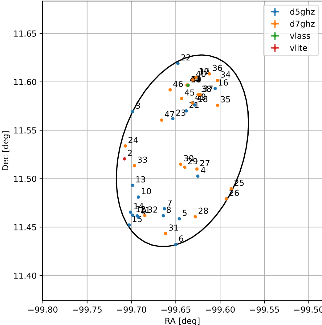
4FGL J1721.4+1131
