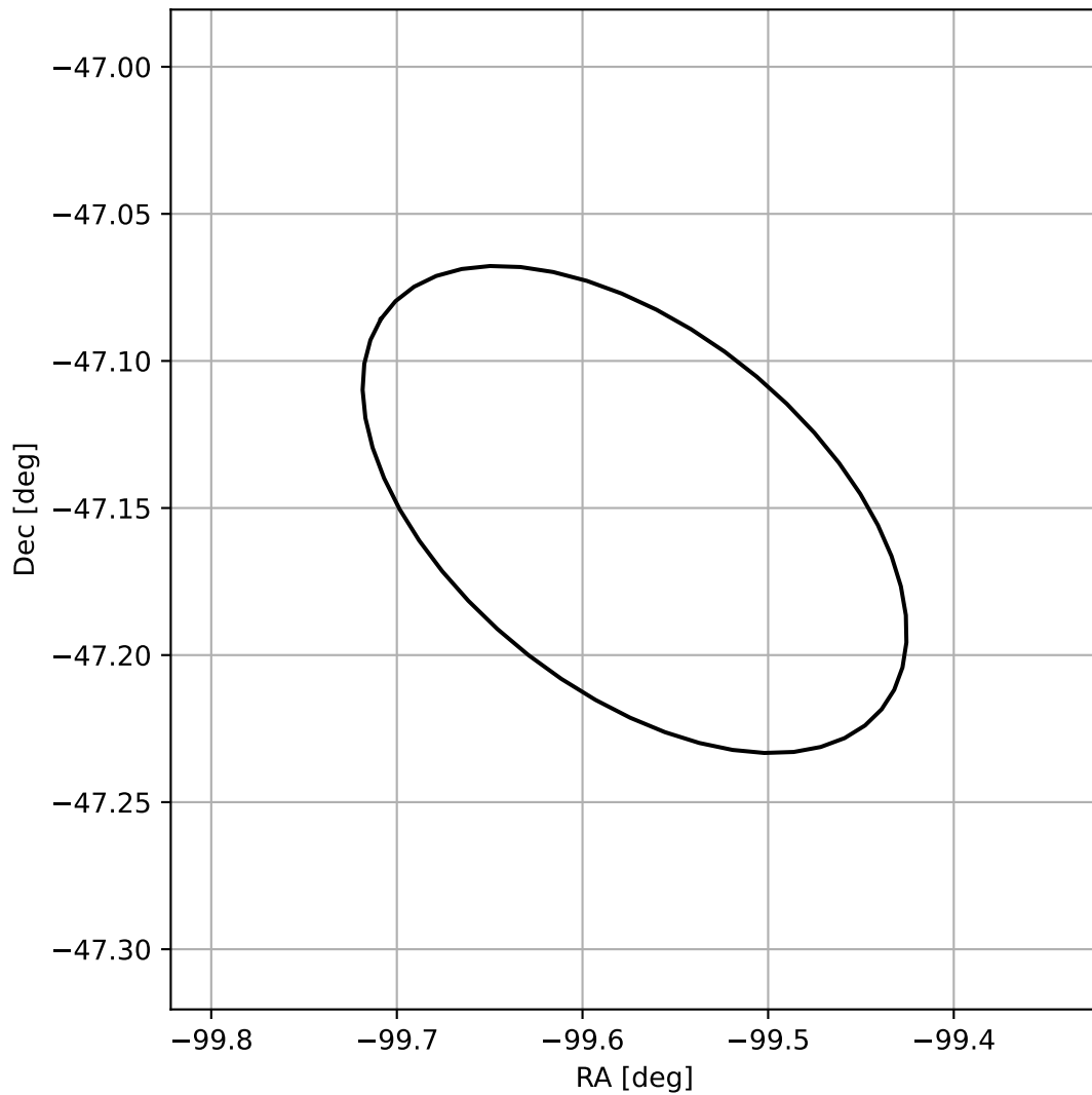
4FGL J1721.7-4709
