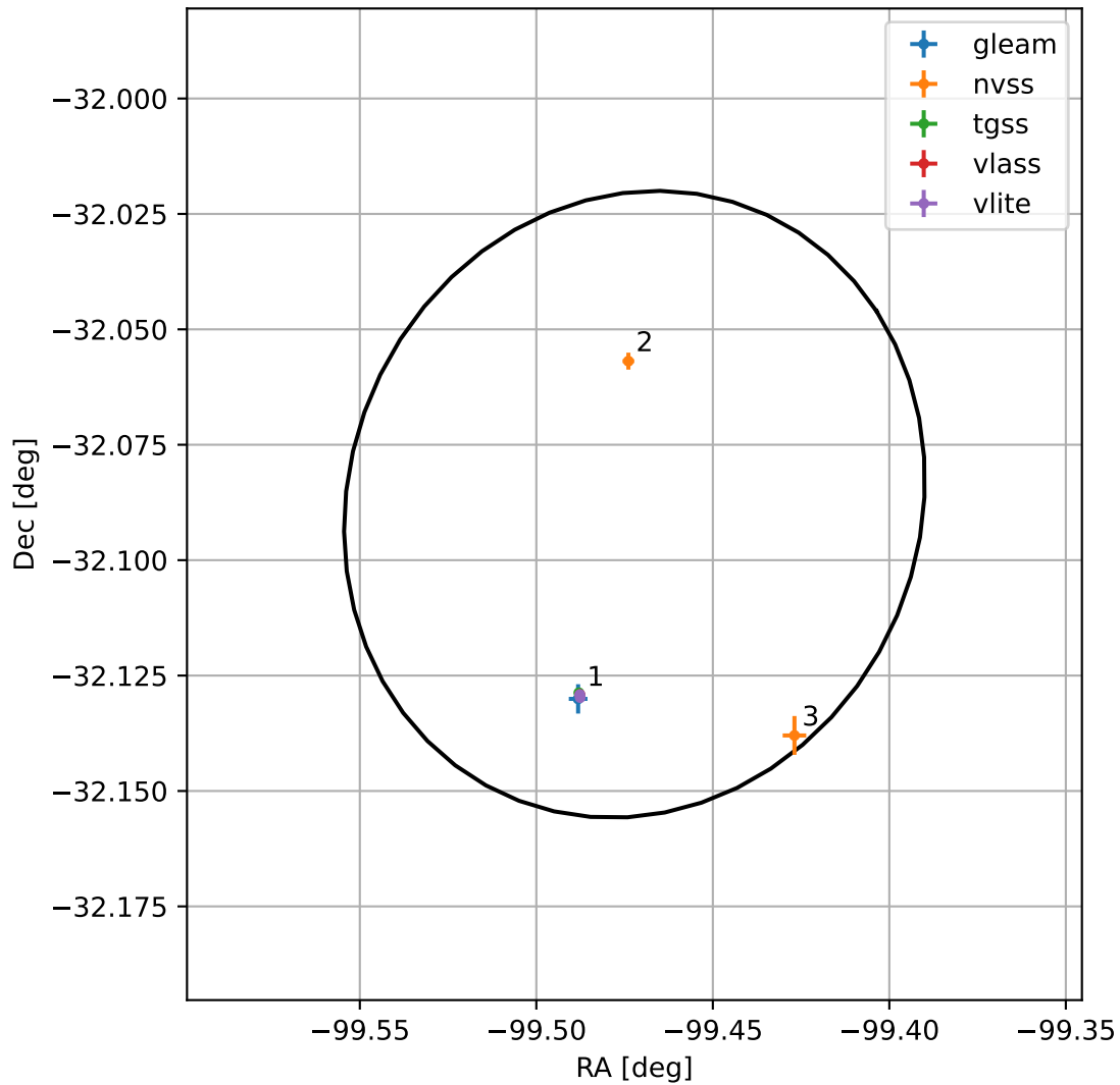
4FGL J1722.1-3205
