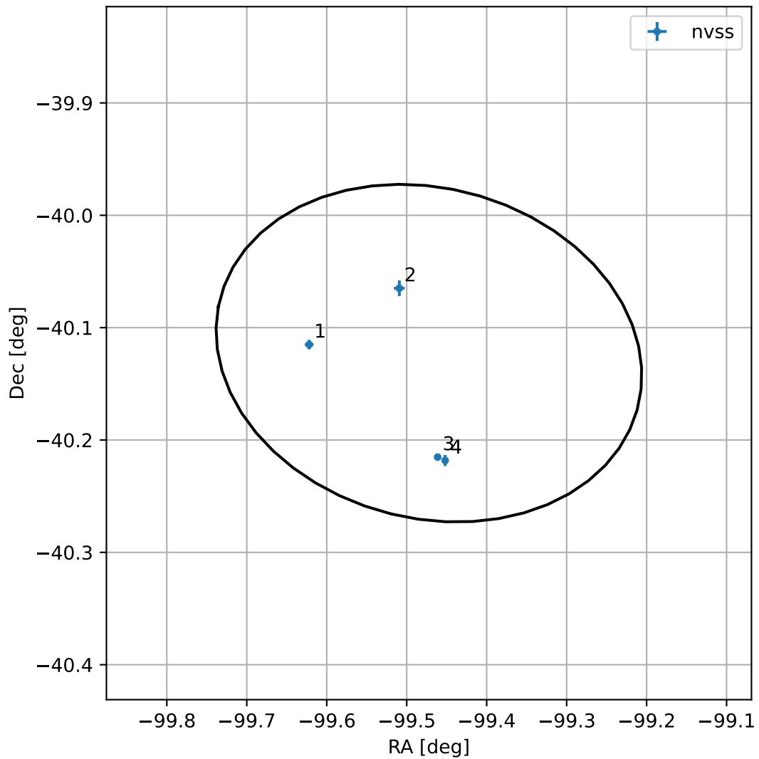
4FGL J1722.1-4007
