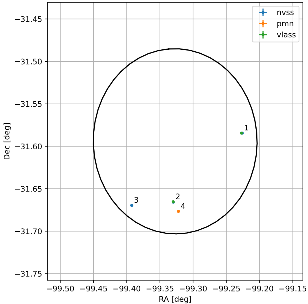
4FGL J1722.6-3135
