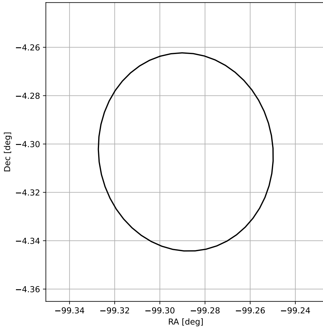
4FGL J1722.8-0418
