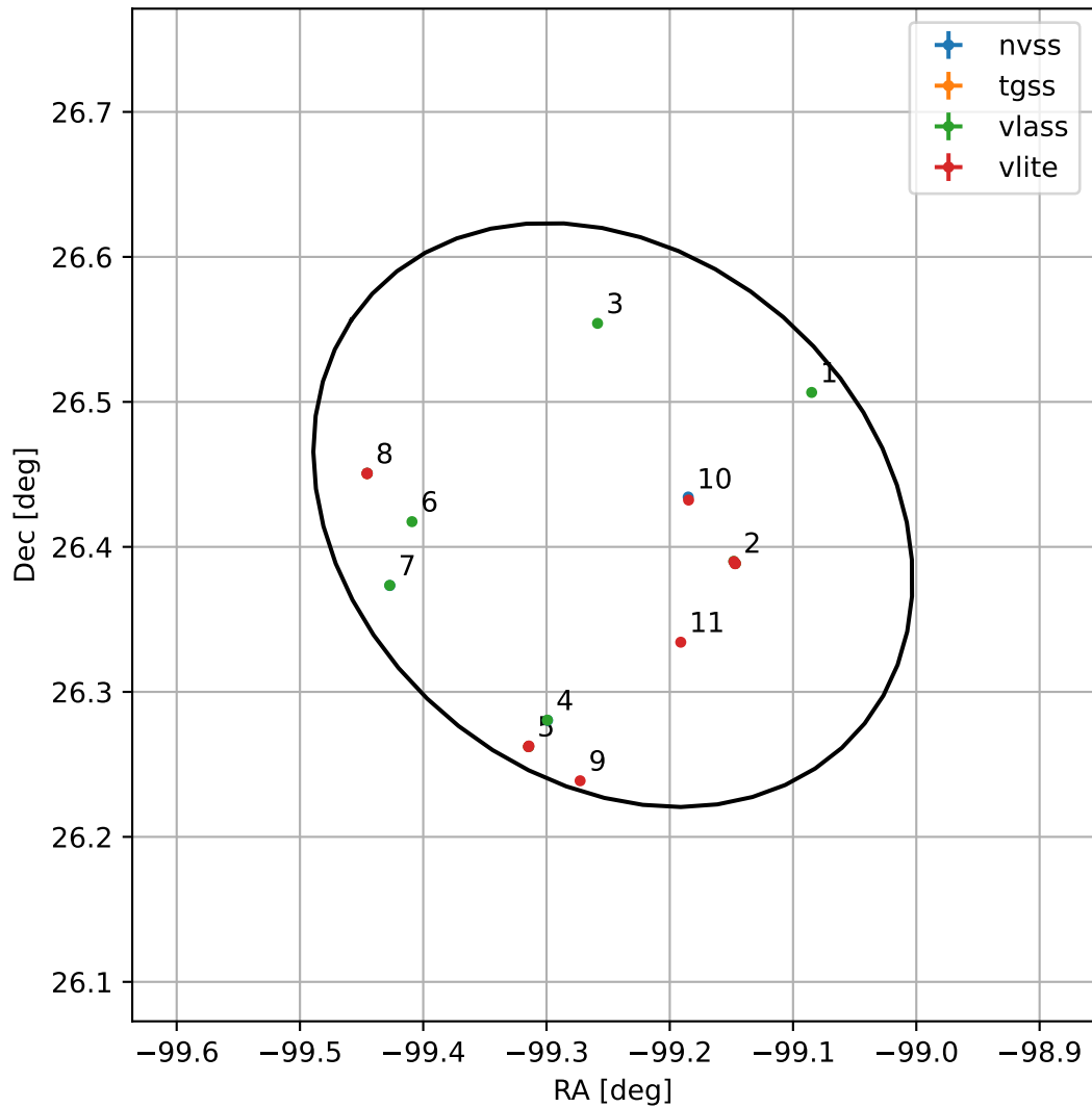
4FGL J1723.0+2625
