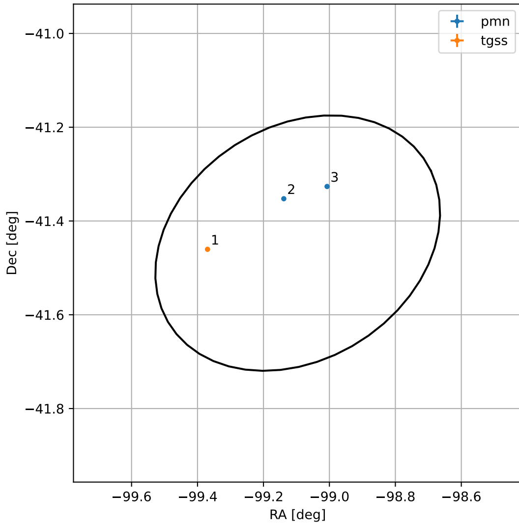
4FGL J1723.6-4126
