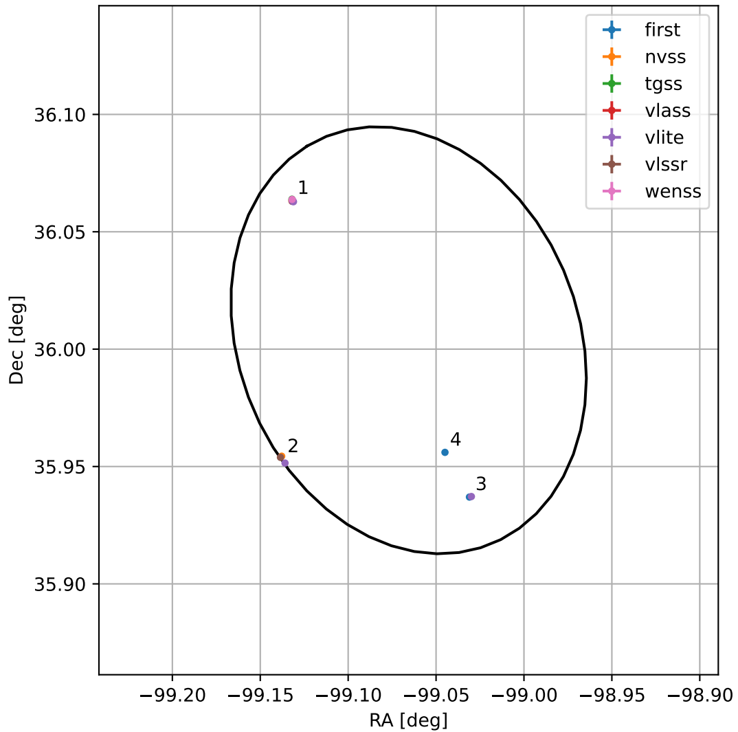
4FGL J1723.7+3600
