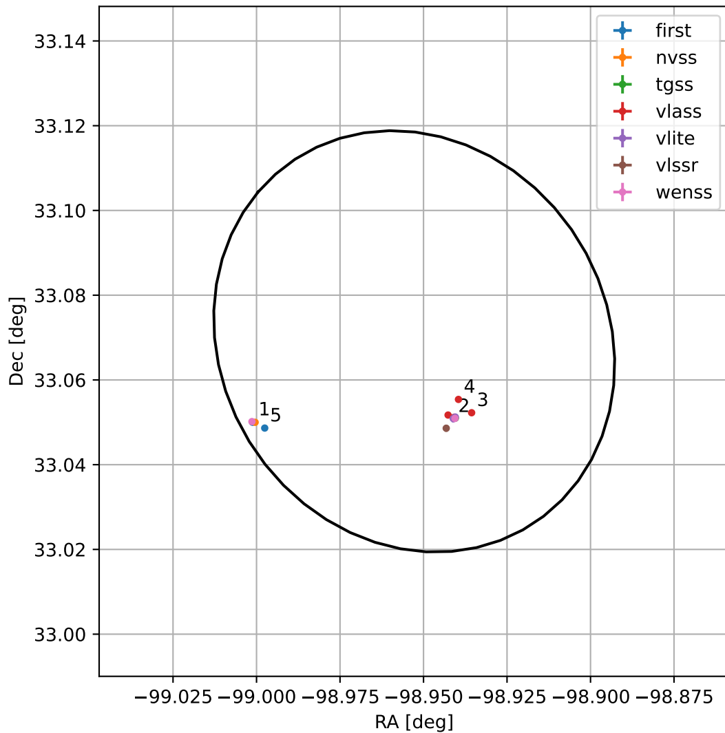
4FGL J1724.1+3304
