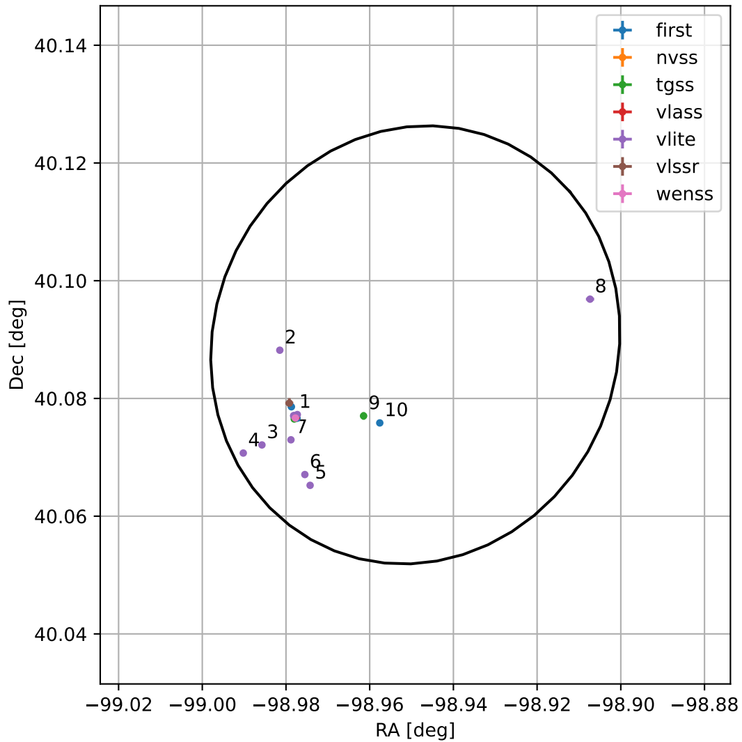
4FGL J1724.2+4005
