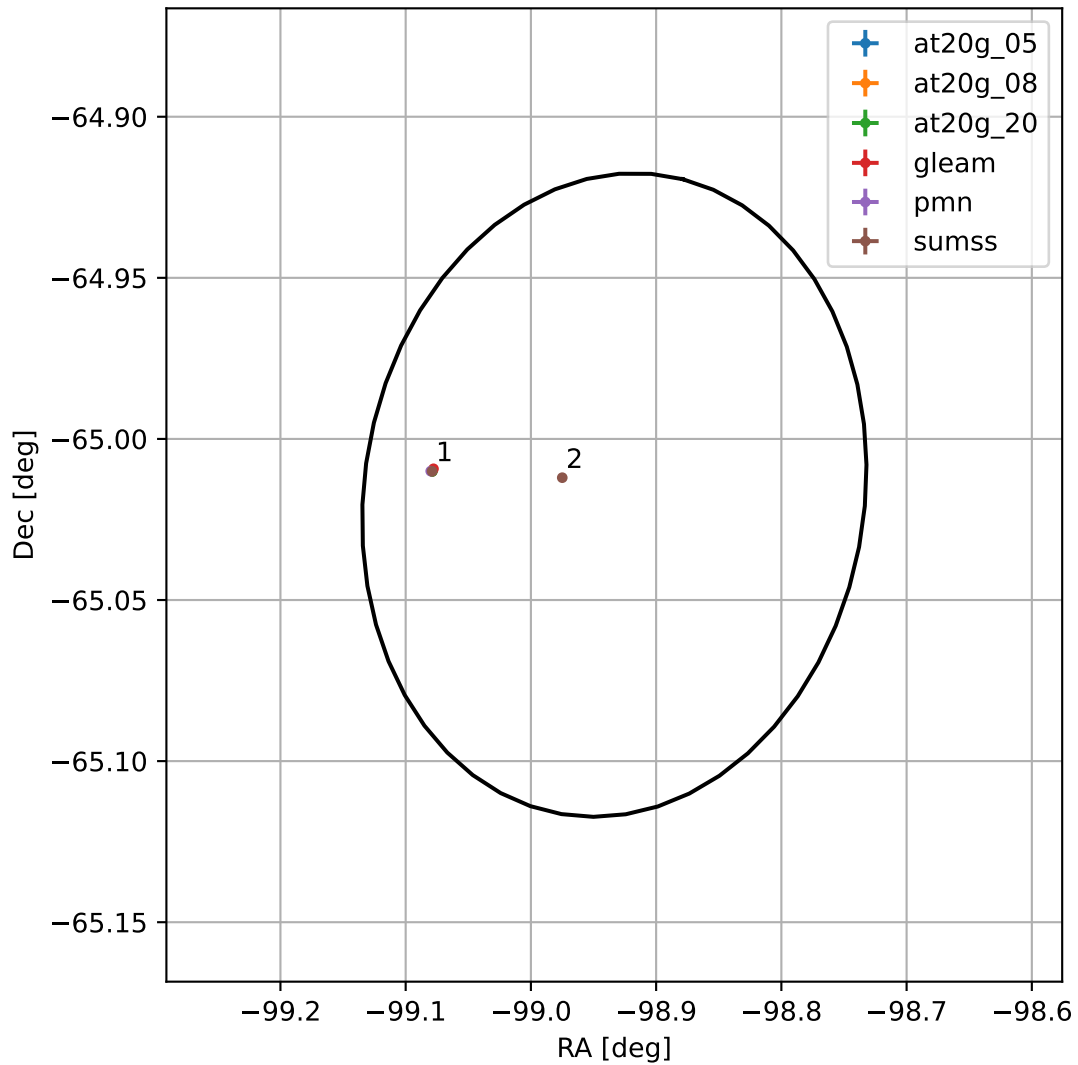
4FGL J1724.2-6501
