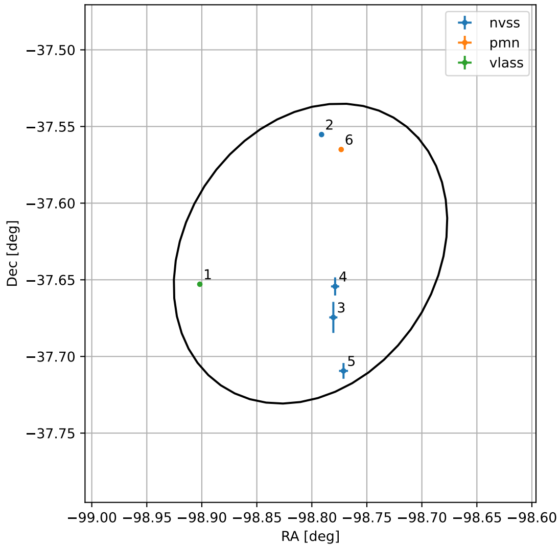
4FGL J1724.7-3737
