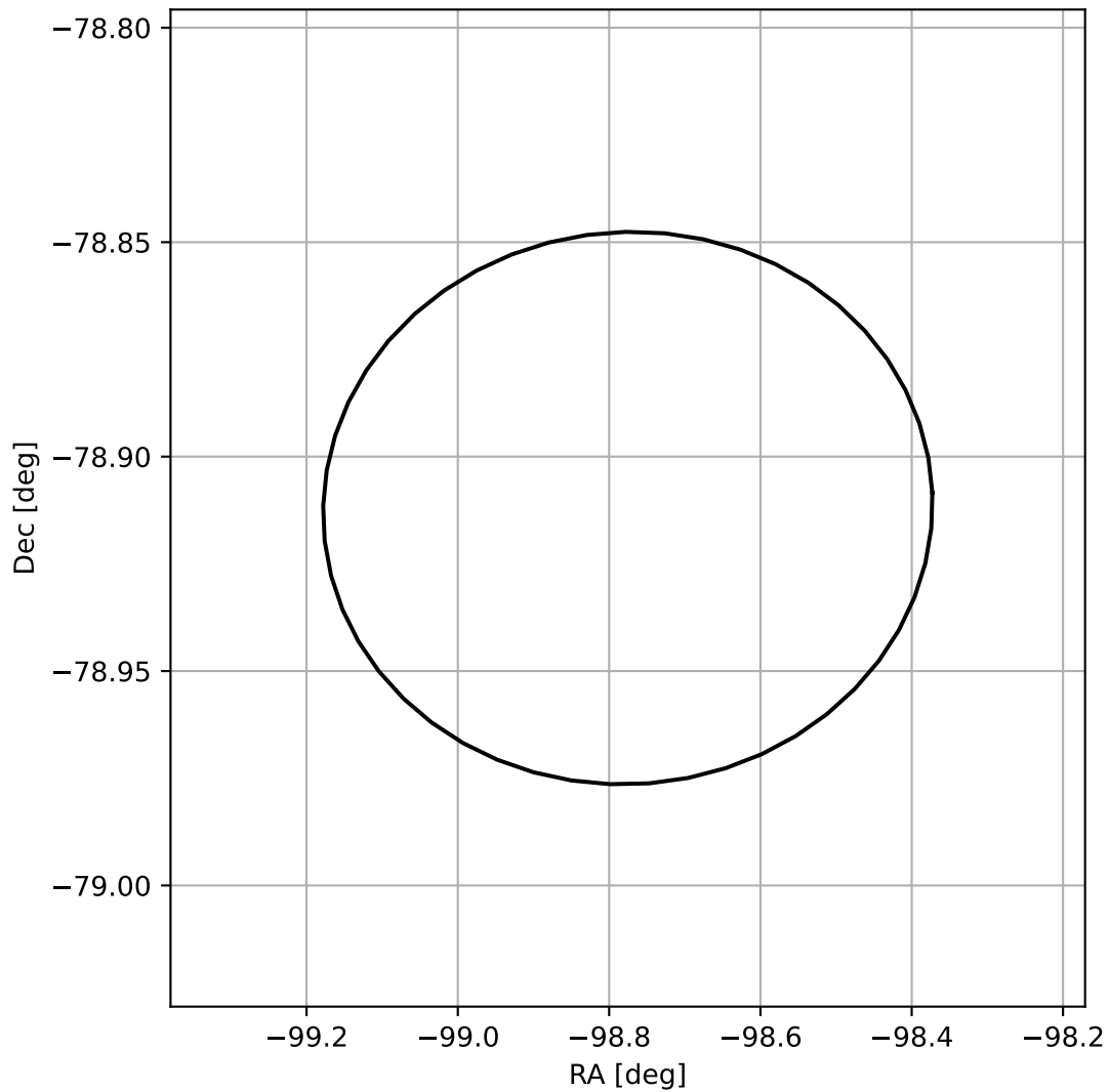
4FGL J1724.8-7854
