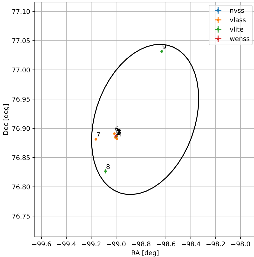
4FGL J1724.9+7654
