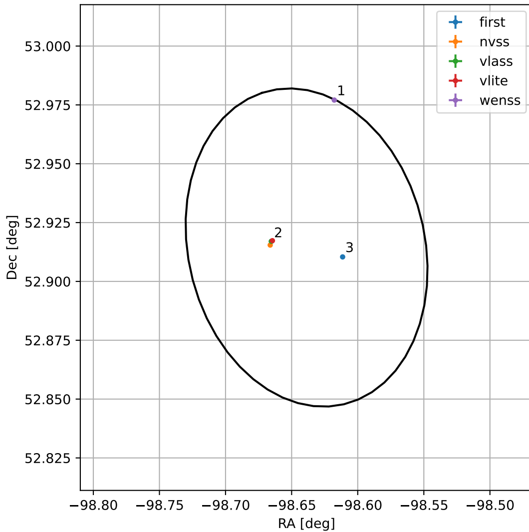
4FGL J1725.4+5254
