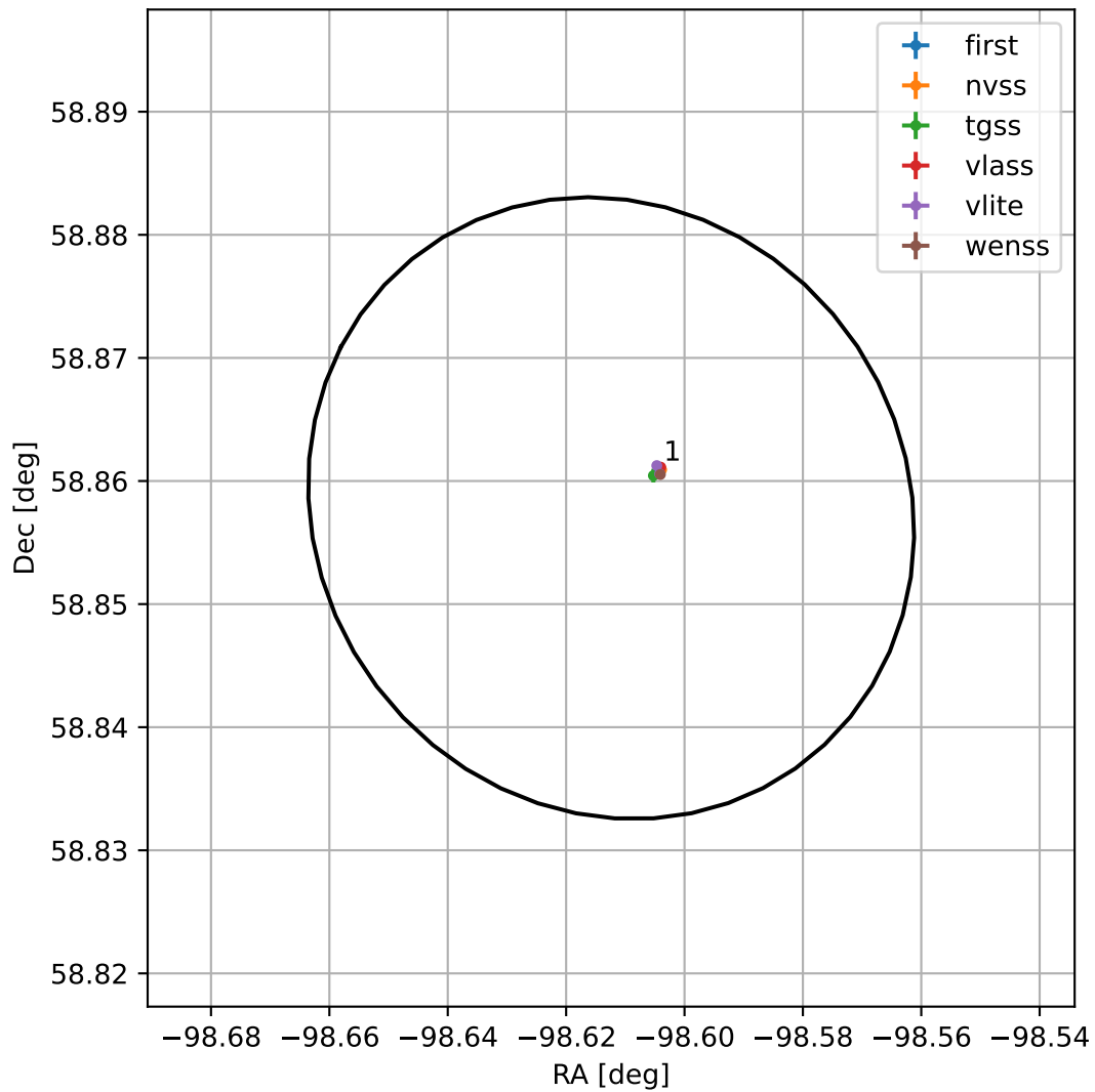
4FGL J1725.5+5851
